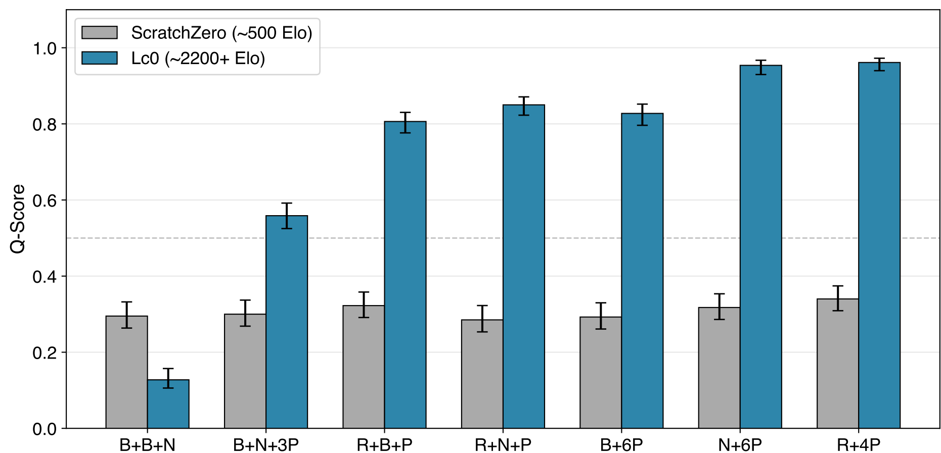
Figure 6: ScratchZero vs Lc0 Comparison
