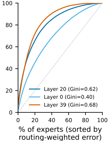
(c) Lorenz curves: expert-level concentration
