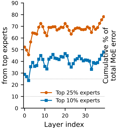
(b) Hot experts dominate MoE output error
