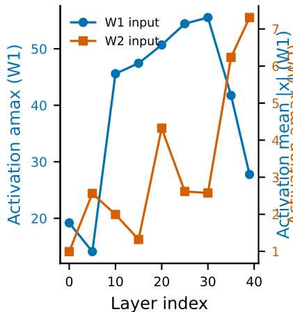
(a) Activation amax by depth
