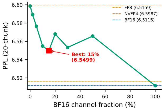
(c) PPL vs BF16 fraction (weight-magnitude selection)
