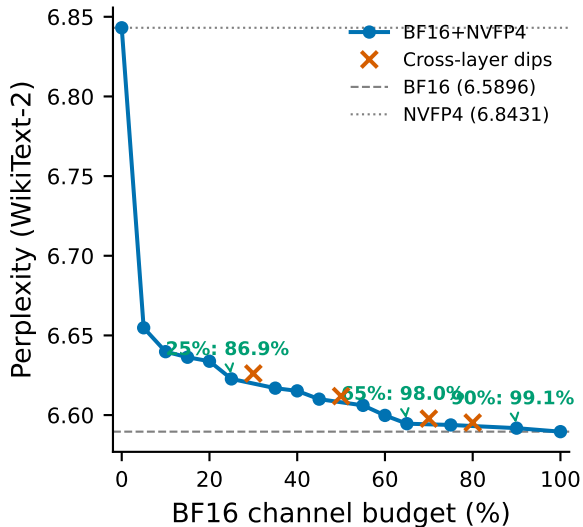
(a) BF16+NVFP4 Pareto Curve
