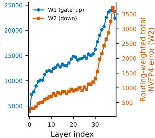
(c) Routing-weighted NVFP4 error by depth (dual axes)
