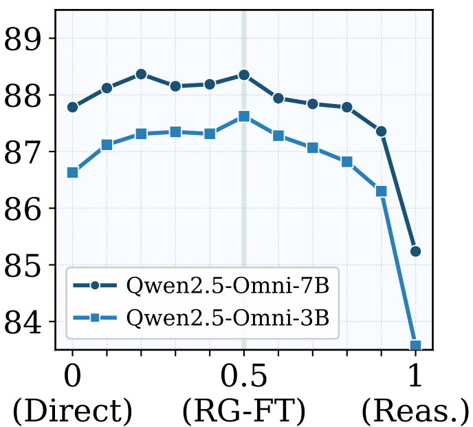
Intent Accuracy
