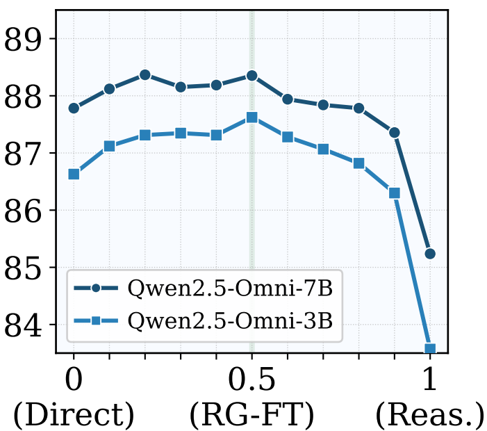
Intent Accuracy
