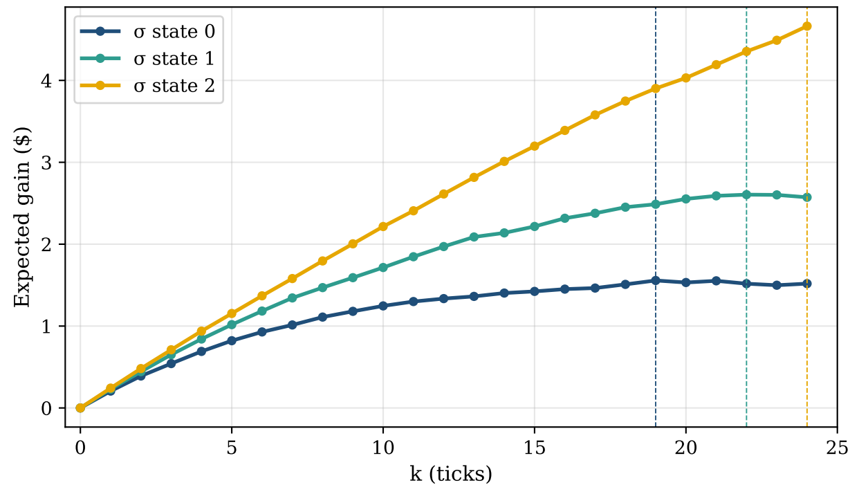
Expected gain k \cdot \varepsilon \cdot P(\text{fill}) — train
