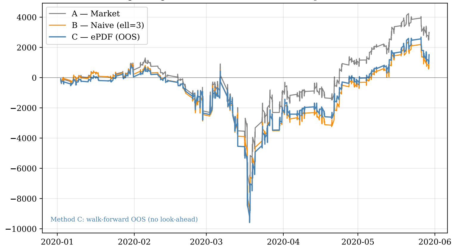
AI Agent signal — Cumulative PnL Nasdaq tau=15 min
