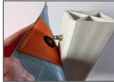
Pin for attaching the sign to the BALIPLAST post
