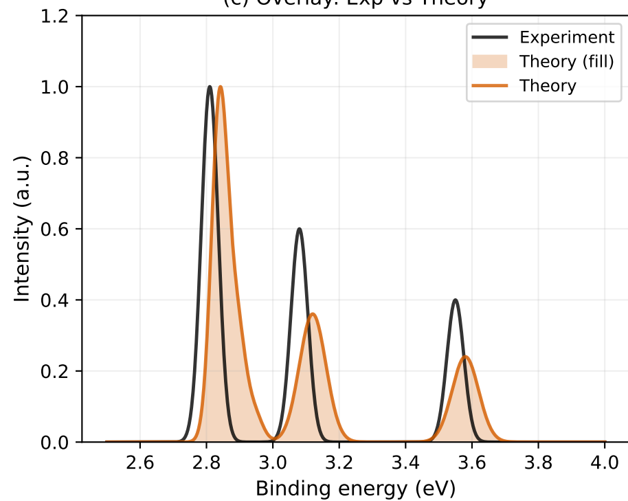
(c) Overlay: Exp vs Theory
