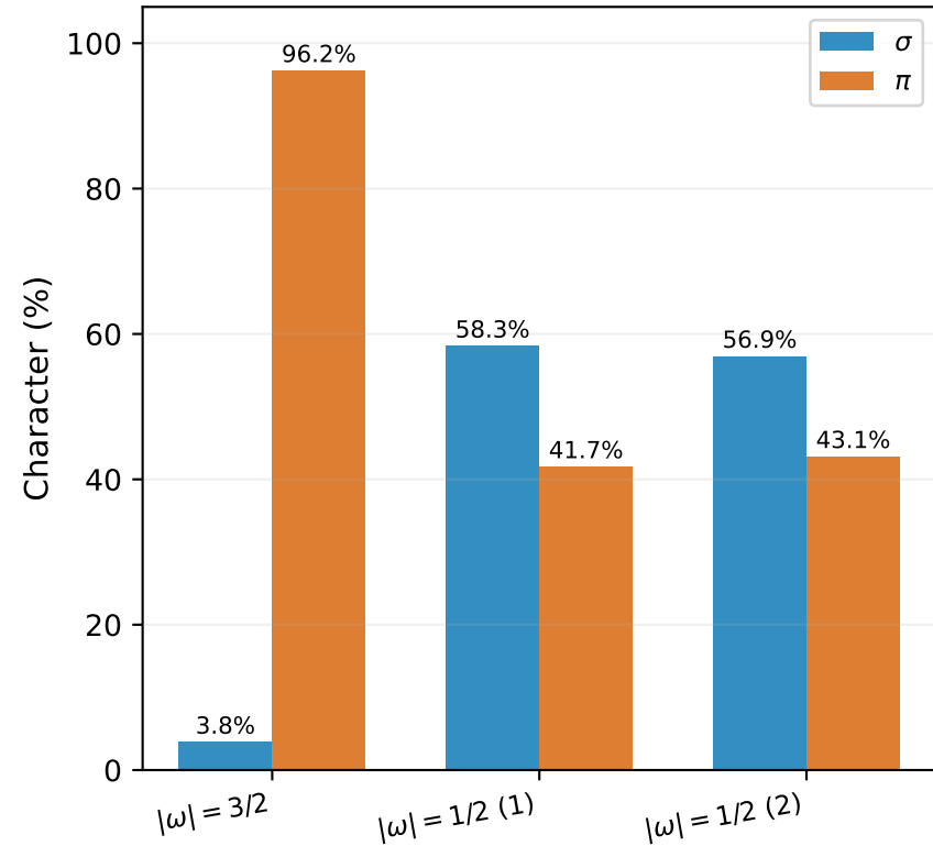
(c) Orbital composition
