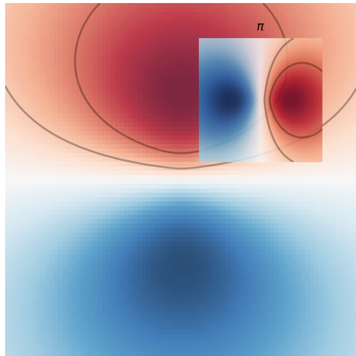
(a) NR: \sigma (cylindrical)
