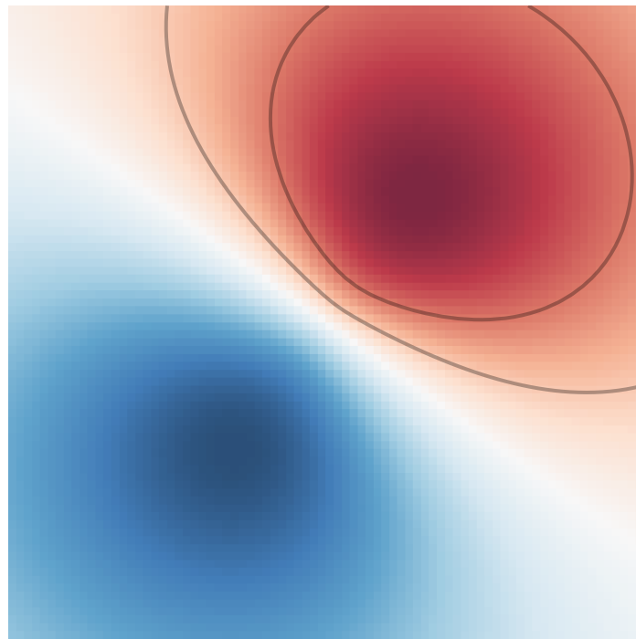
(b) Relativistic: |\omega| = 1/2
