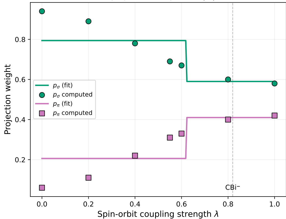
(b) \sigma/\pi projection weights for |\omega|=1/2
