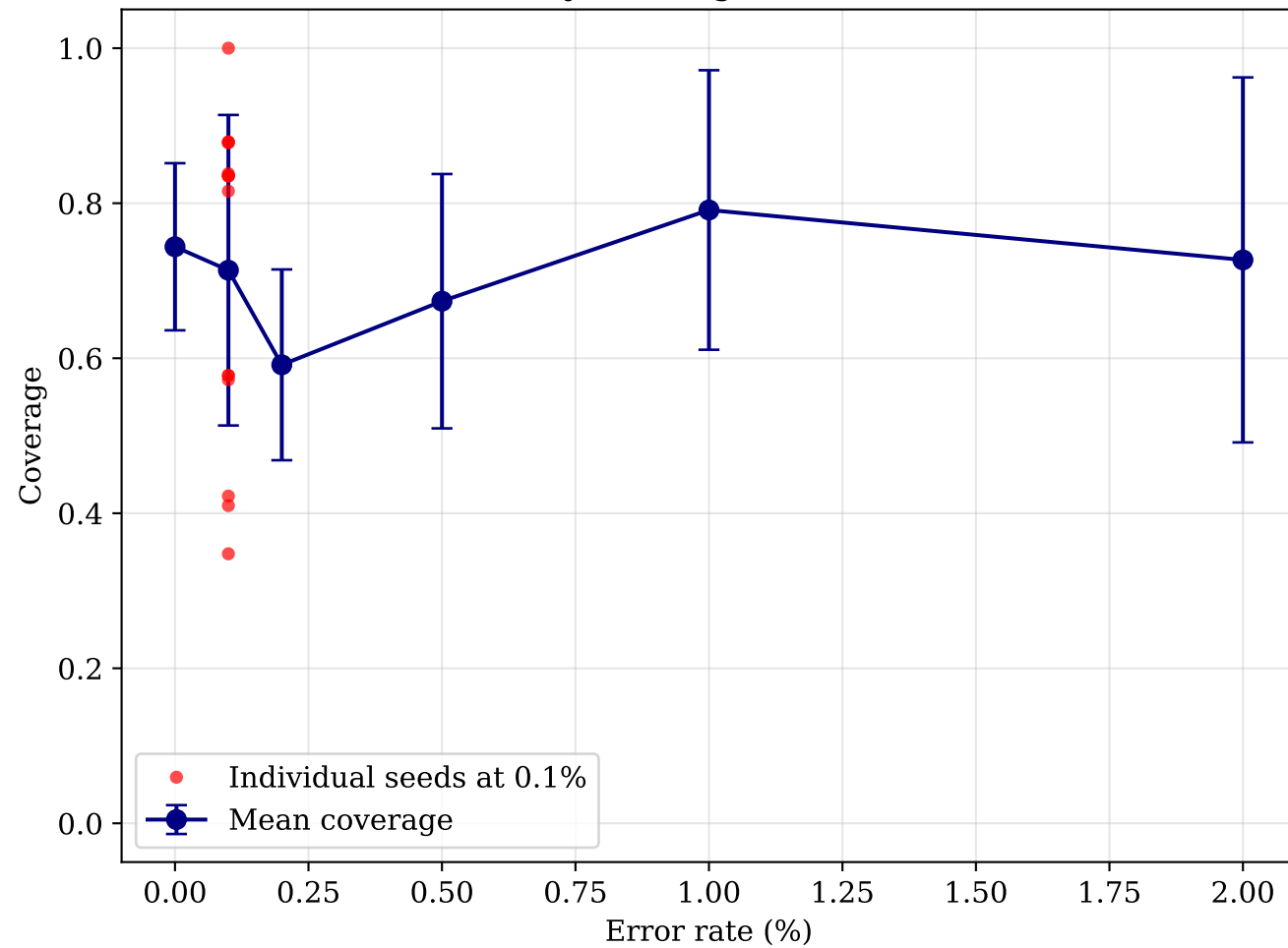
Assembly coverage vs. error rate
