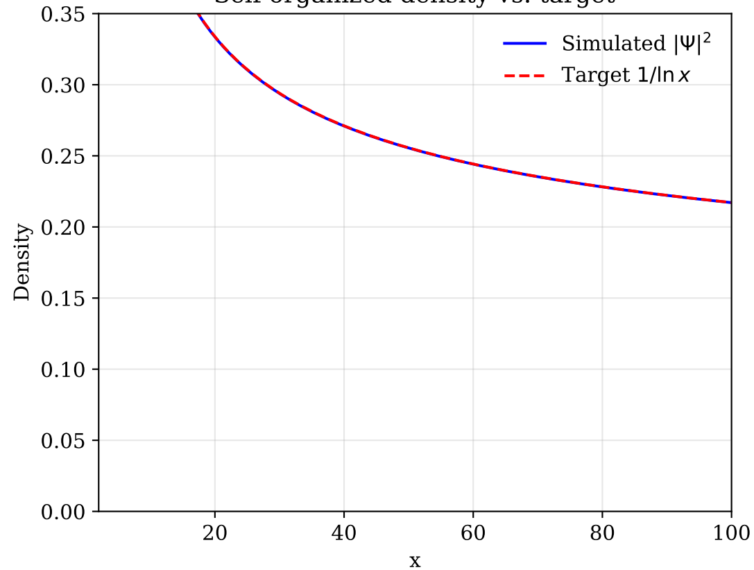
Self-organized density vs. target
