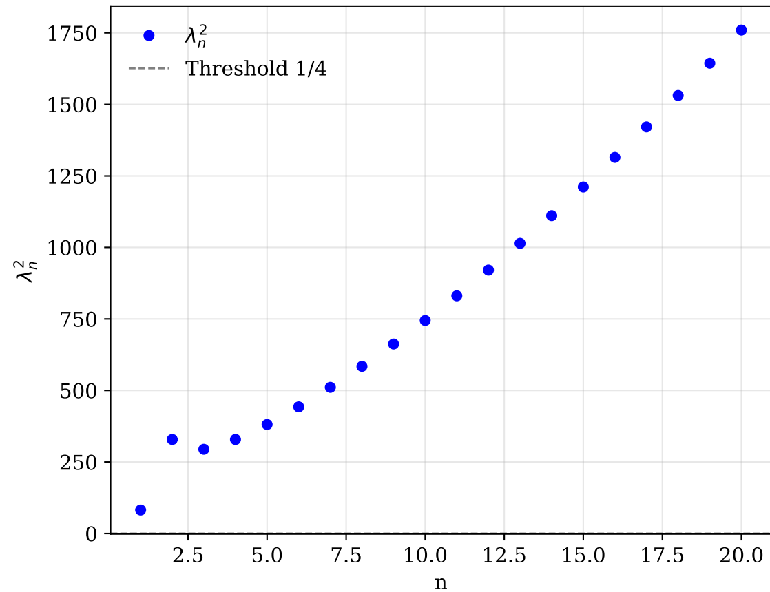
Spectrum of \Delta_K
