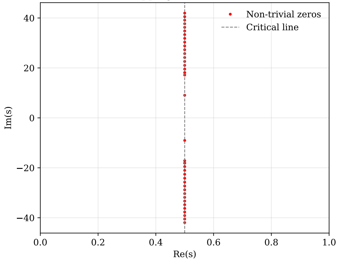
Mapping to zeta zeros
