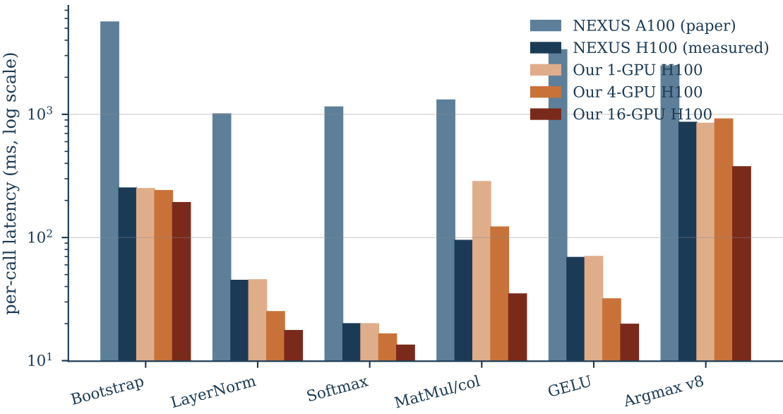
Per-op latency: NEXUS published vs measured-on-H100 vs multiNEXUS
