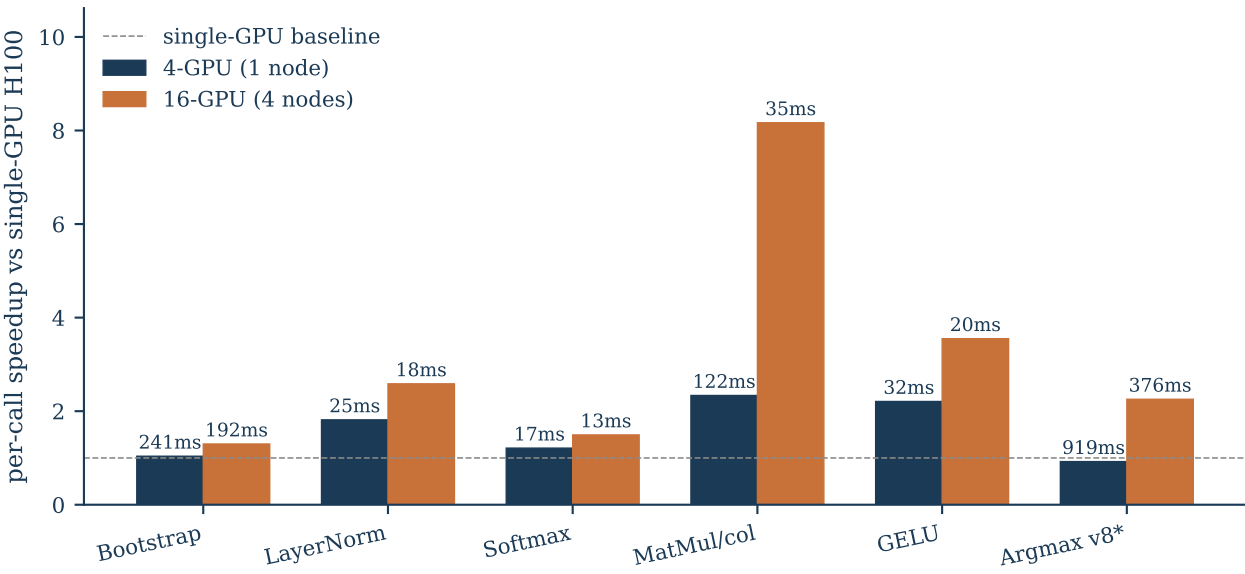
Multi-GPU per-op latency speedup (NEXUS-aligned parameters)
