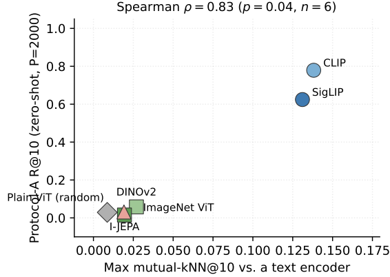
Figure 4. Each point is one image encoder. The x -axis is its maximum mutual- k NN@10 against the four text encoders (column max of Table 4); the y -axis is its zero-shot Protocol-A R@10 (Table 1). Marker shape and pastel colour code the pretraining family. Spearman \rho = 0.83 ( p = 0.04 , n = 6 ).
