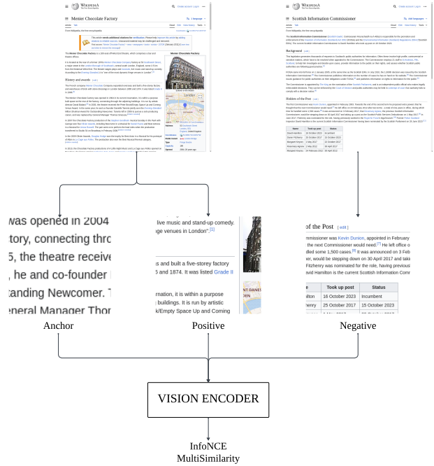
Figure 3. Training. Each step samples four pages \times four crops; same-page crops are positives, cross-page crops are negatives. The image encoder produces an L2-normalised descriptor; training minimises a multi-similarity contrastive loss (Wang et al., 2019). We unfreeze the last four ViT blocks (of twelve) and train a head on top.
