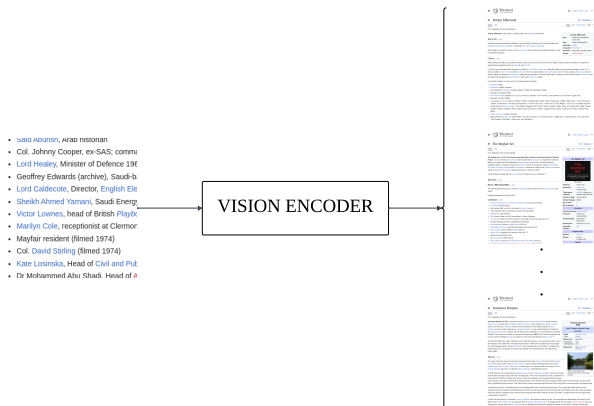
Figure 2. Anchor-pool benchmark (Phase 2). Each anchor crop is encoded with the vision encoder and ranked against a small pool ( \sim 7 images) of positives (other crops of the same page) and hard negatives (crops of unrelated pages).
