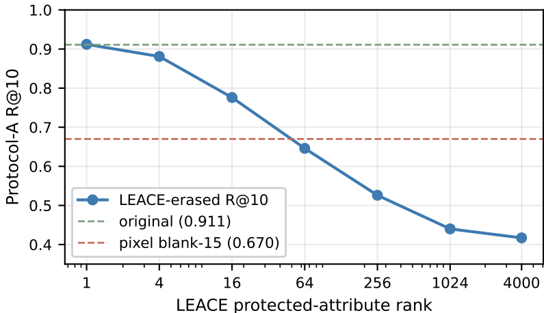
trained DINOv2-SALAD-50k: rank-64 LEACE matches blanking
