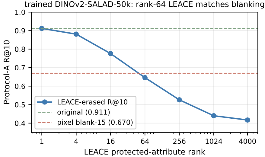
Figure 6. LEACE rank sweep on trained DINOv2-SALAD-50k (§4.7). The Protocol-A R@10 of the LEACE-erased descriptors is plotted against the rank of the protected attribute Z . The pixel-blanking delta ( -0.241 , dashed orange) is matched at rank \approx 64 , indicating the trained title-region binding lives in a 16–64-dim subspace of the 8 448-d SALAD descriptor.
