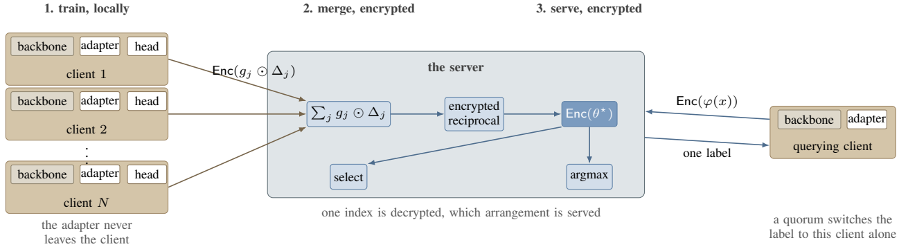
Fig. 1. The protocol in three stages. Each client fine-tunes an adapter and a classifier head on the same frozen public backbone, keeps the adapter, and uploads one encrypted head displacement weighted by its per-class counts. The server adds the ciphertexts and divides by the per-class totals under encryption, holding no decryption key, so the shared head \theta^* exists only as a ciphertext. The same server answers queries.
