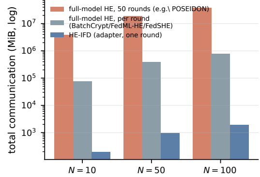
Fig. 3. Total communication on a shared backbone (RoBERTa-base), calculated for CKKS ring 2^{14} (0.5 MiB per ciphertext; 50 rounds for the iterative schemes). HE-IFD encrypts only the adapter and runs once; full-model encrypted schemes move gigabytes per round (BatchCrypt, FedML-HE, FedSHE) to terabytes over training (POSEIDON-style encrypted training).
