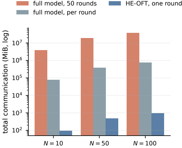
Fig. 3. Total communication on a shared backbone (RoBERTa-base), calculated for CKKS ring 2^{14} (0.5MiB per ciphertext; 50 rounds for the iterative schemes). HE-OFT encrypts only the adapter and runs once; full-model encrypted schemes move gigabytes per round (BatchCrypt, FedML-HE, FedSHE) to terabytes over training (POSEIDON-style encrypted training).
