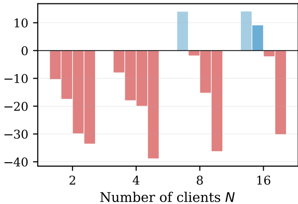
Fashion-MNIST
