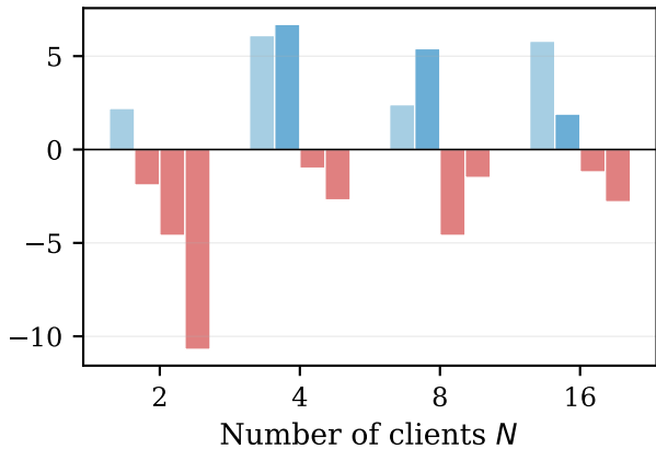
CIFAR-10
