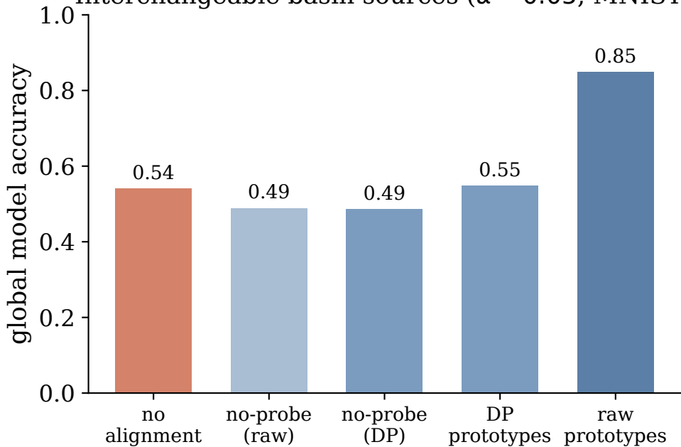
Interchangeable basin sources ( \alpha = 0.05 , MNIST)
