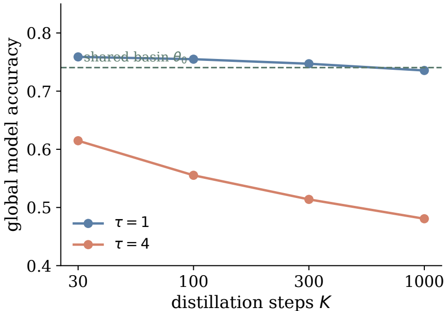
Bounded trajectories: short is best, long drifts away (ResNet-18, CIFAR-10)
