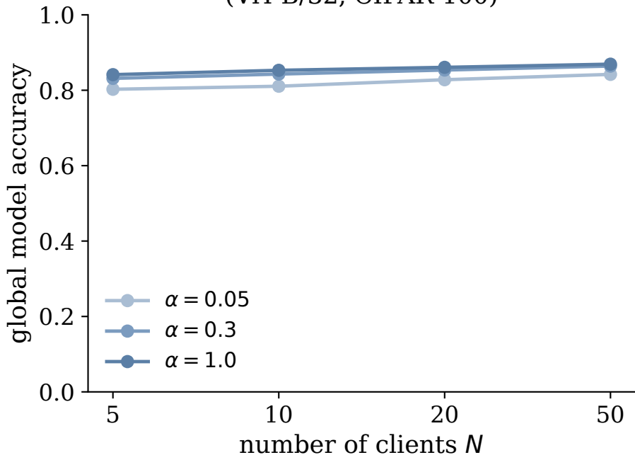
Accuracy is stable as the client count grows (ViT-B/32, CIFAR-100)
