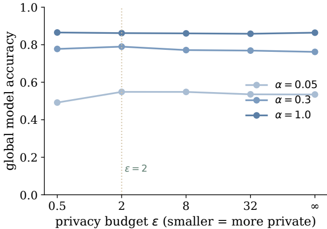
Fig. 8. The privacy–utility frontier on the basin prototypes is flat across the practical privacy regime. Tightening the differential-privacy budget on the per-class summaries through the single-digit \epsilon typical of differentially private learning leaves the global model’s accuracy essentially unchanged; it falls only under the most stringent budget, \epsilon = 0.5 (MNIST, N = 10 ).
