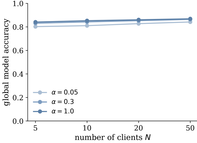
Fig. 5. The global model’s accuracy is stable as the number of clients grows from 5 to 50 (ViT-B/32, CIFAR-100), at every heterogeneity level.
