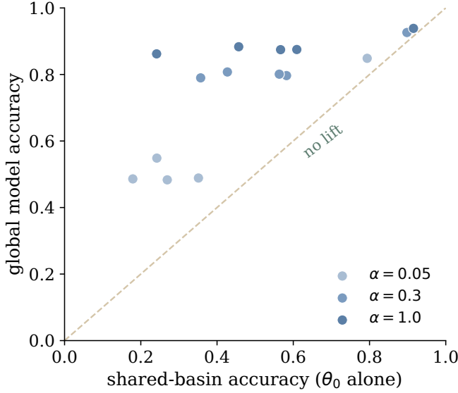
Fig. 7. Distillation never hurts and adds most where the basin is weak. Each point is a basin source at a given heterogeneity \alpha (MNIST, N = 10 ); the horizontal axis is the accuracy of the shared basin \theta_0 on its own and the vertical axis the accuracy of the resulting global model. All points lie above the no-lift diagonal, and the gap is largest when the basin is weakest.
