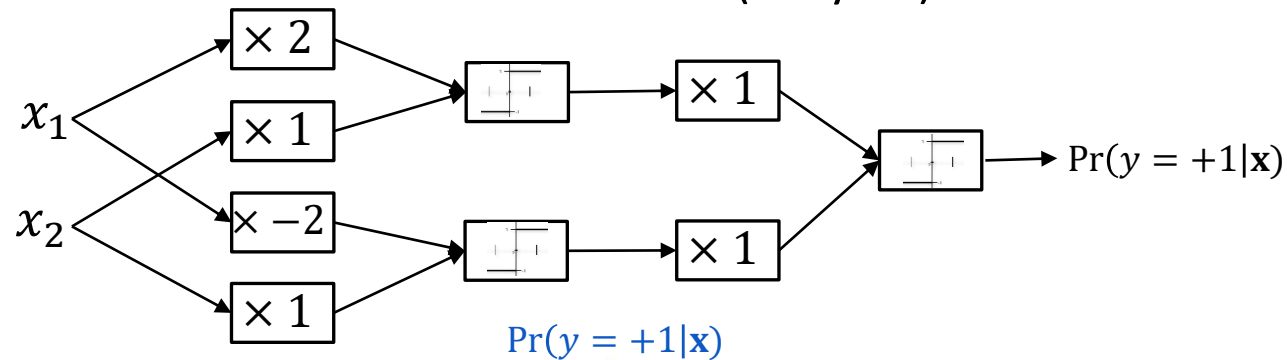
Neural network (2 layers)
