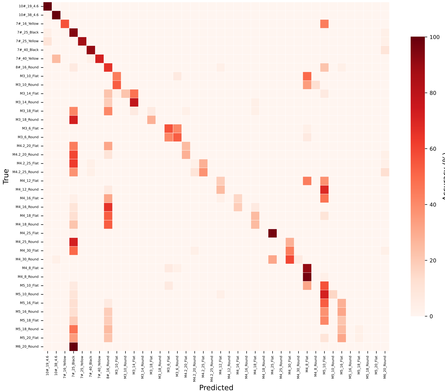
ConvNeXt-Tiny — Shadow (worst, 33.0%)
