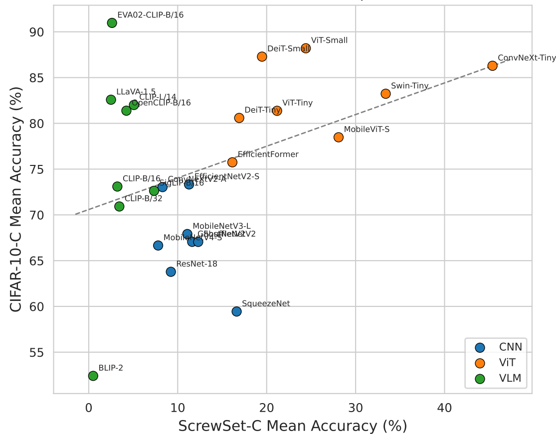
SS-C vs CIFAR-10-C ( r=0.391 , p=5.861e-02 )
