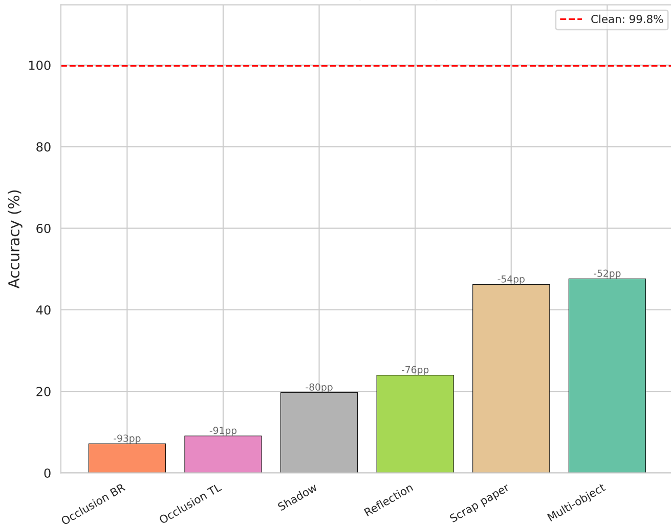
ViT: Per-Corruption Accuracy (sorted by difficulty)
