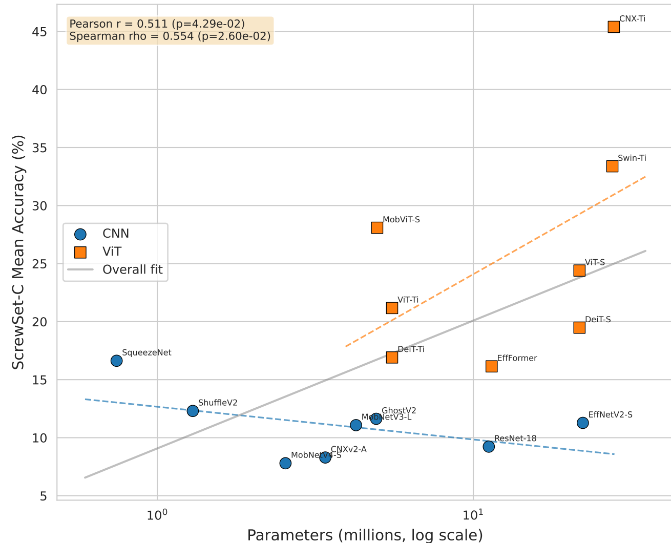
A2. Supervised Models Only
