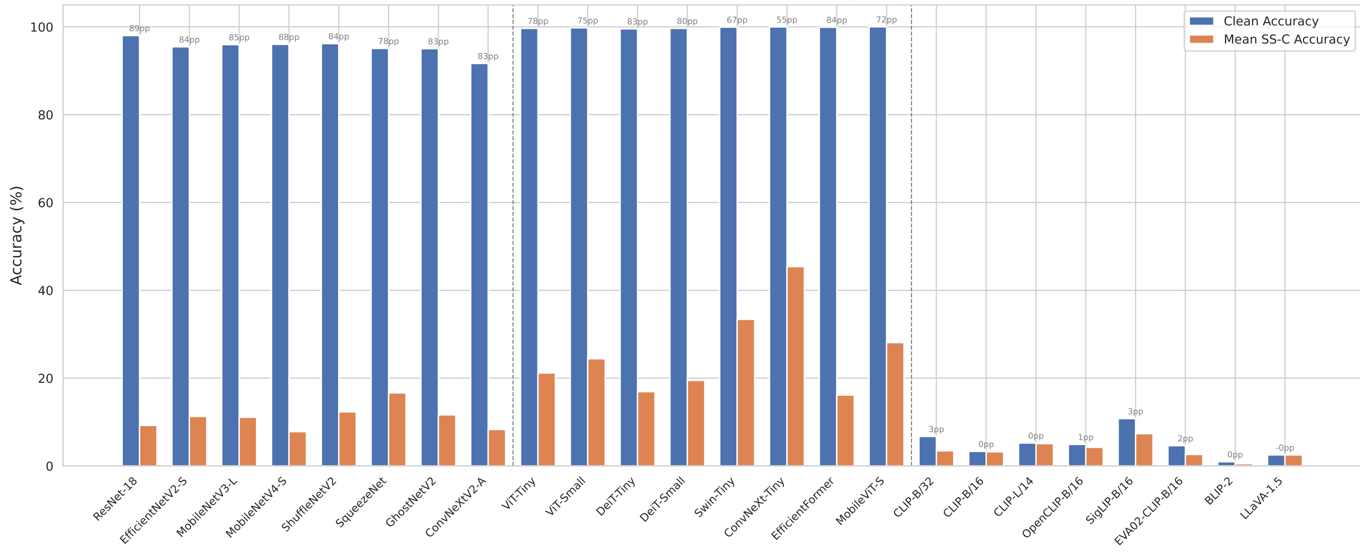
ScrewSet: Clean vs Corruption Accuracy Gap
