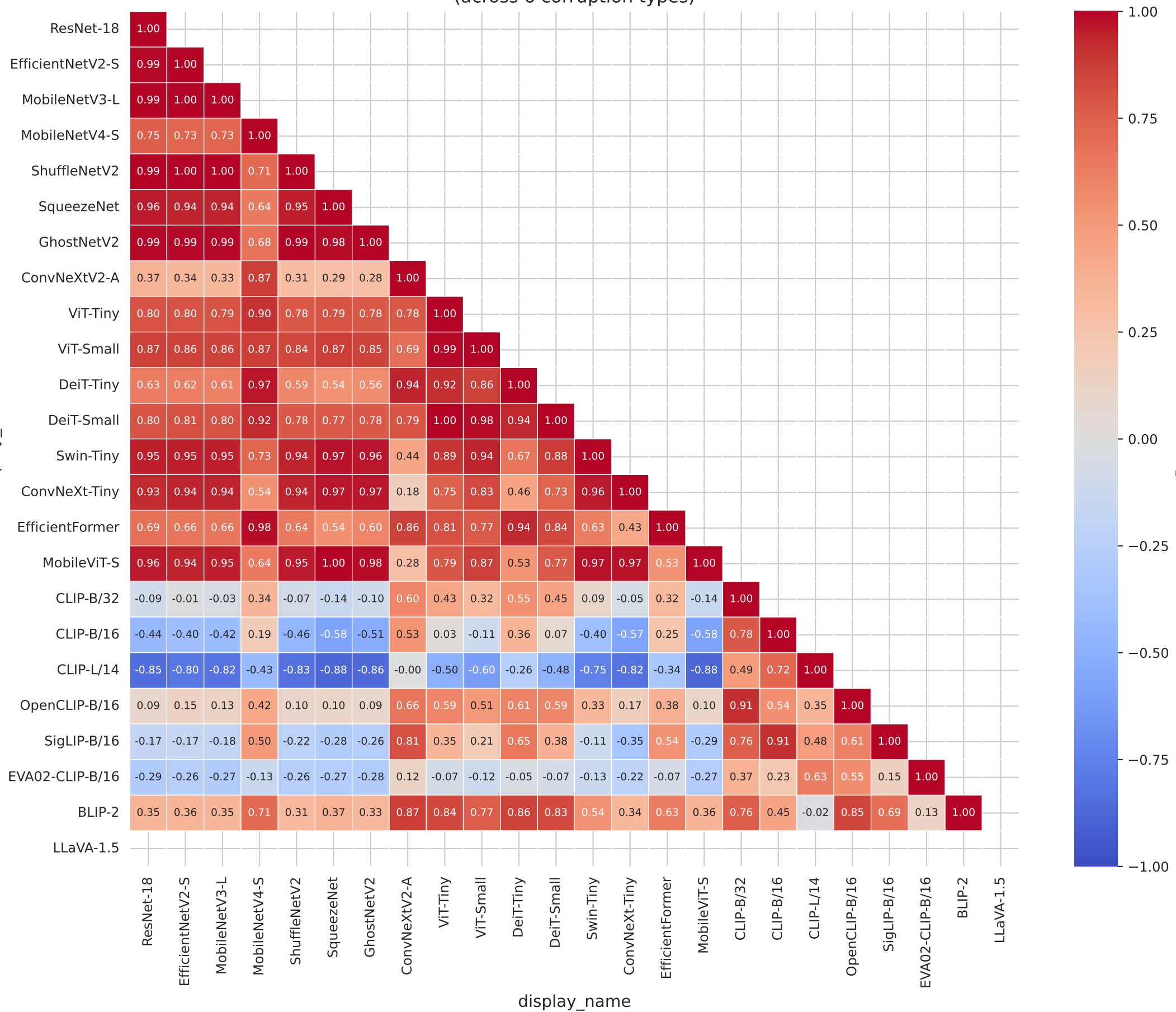
ScrewSet-C: Model-Model Correlation (across 6 corruption types)
