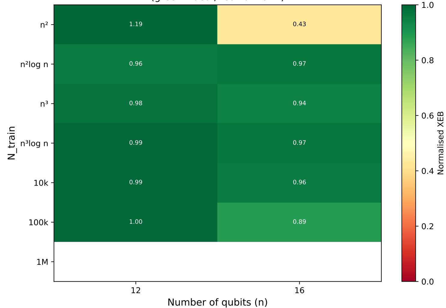
RNN: Normalised XEB heatmap (green=ideal, red=uniform)
