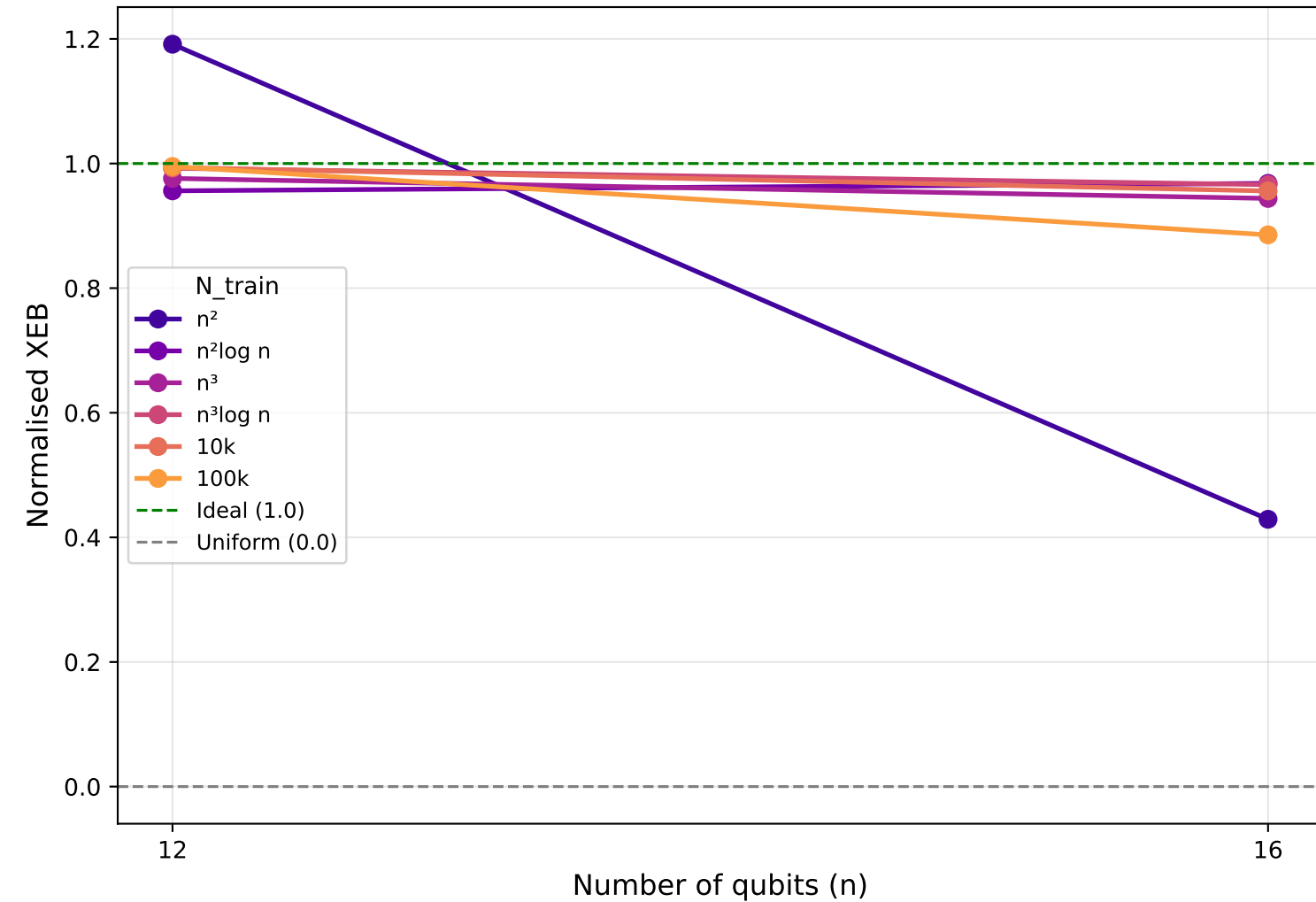
RNN: XEB vs n — one curve per N_train
