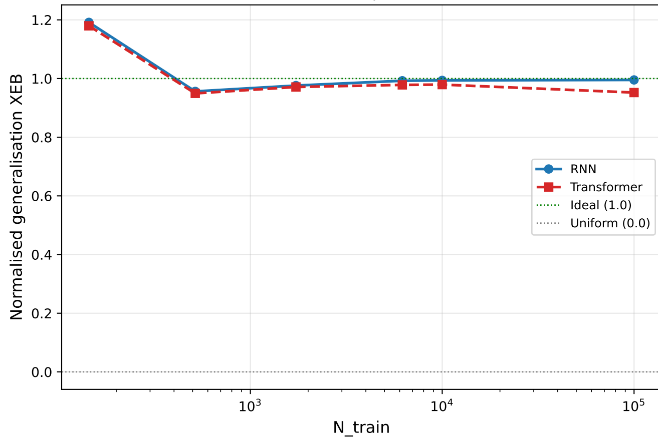
n = 12 qubits
