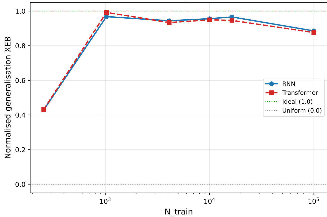
n = 16 qubits
