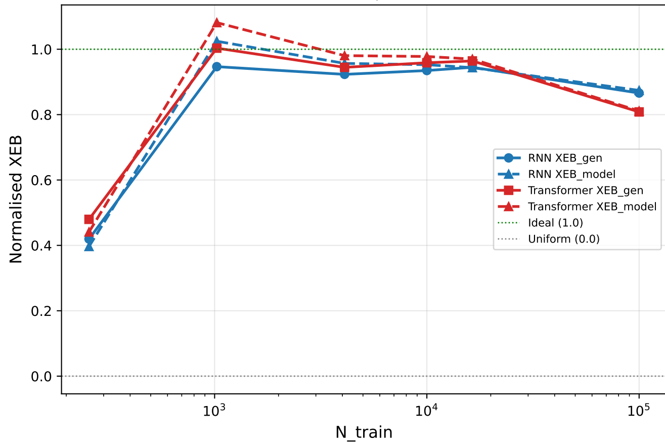
n = 16 qubits
