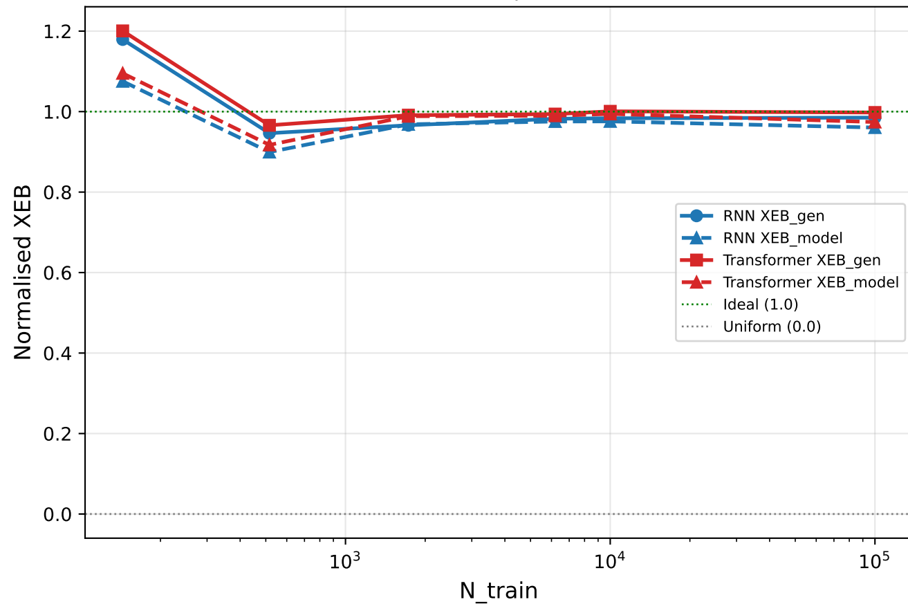
n = 12 qubits
