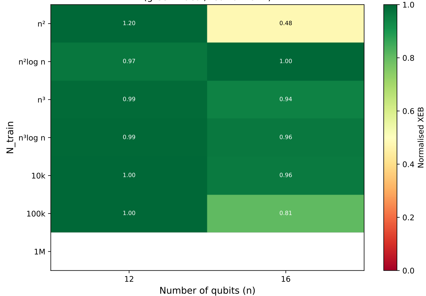
Transformer: Normalised XEB heatmap (green=ideal, red=uniform)
