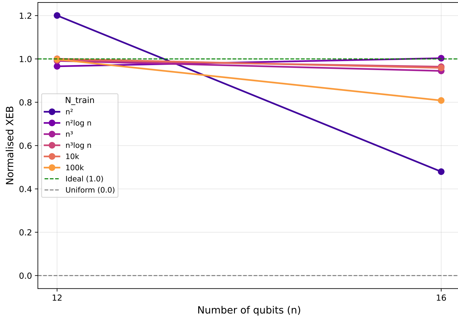
Transformer: XEB vs n — one curve per N_train
