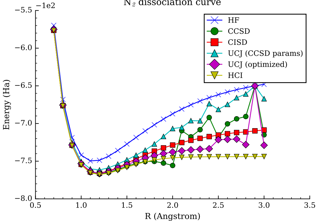
N_2 dissociation curve
