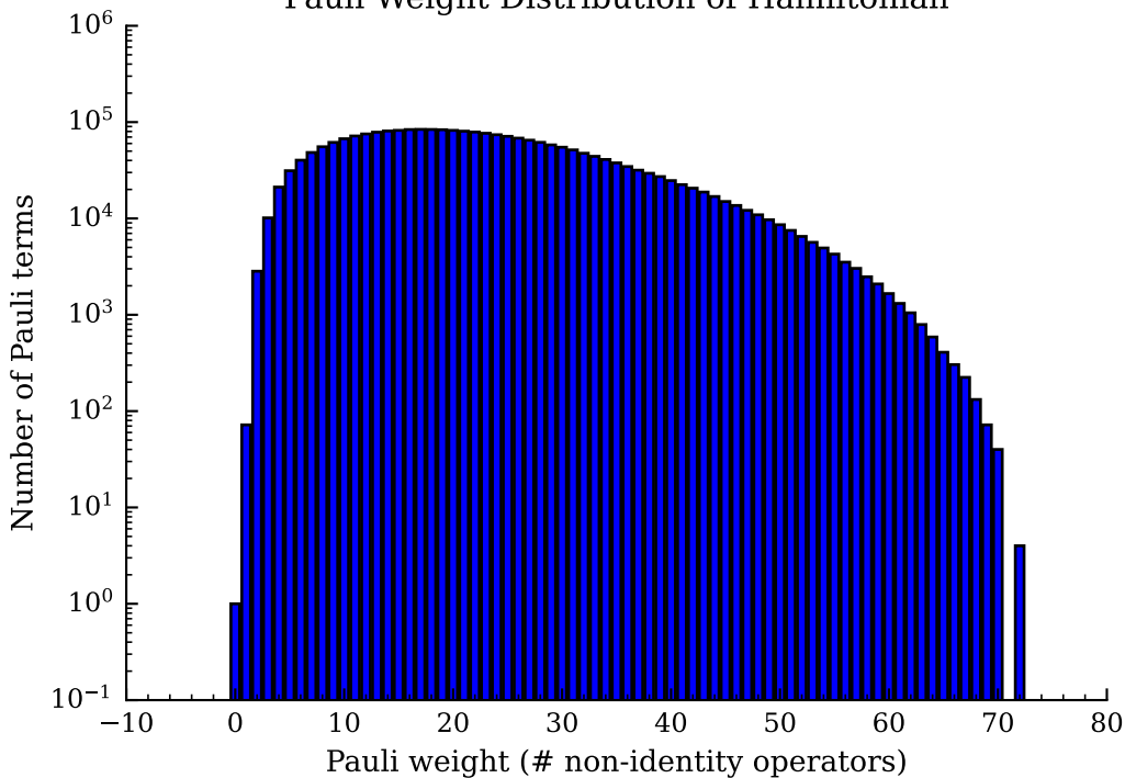
Pauli Weight Distribution of Hamiltonian
