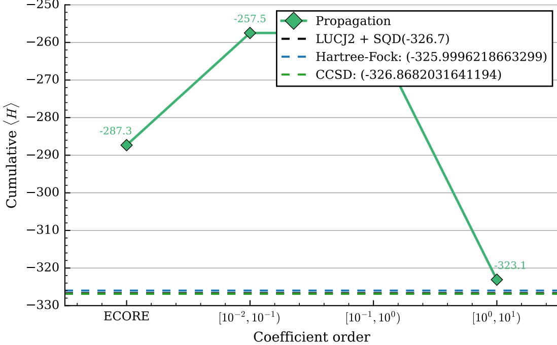
Cumulative Expectation Value by Coefficient Order for noiseless FeS LUCJ ansatz propagation
