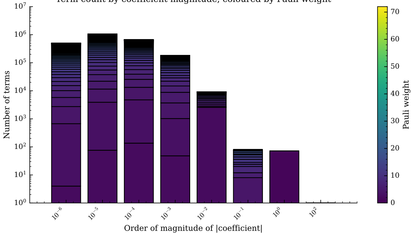
Term count by coefficient magnitude, coloured by Pauli weight
