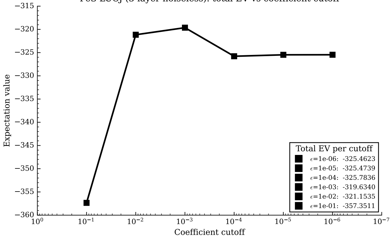
FeS LUCJ (3-layer noiseless): total EV vs coefficient cutoff
