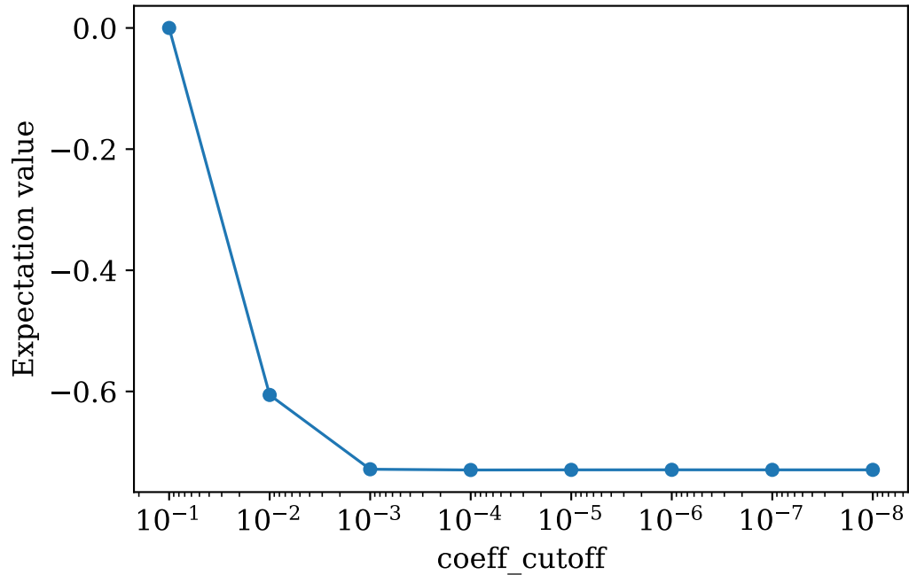
Z-string (w=1), damping=0.001
