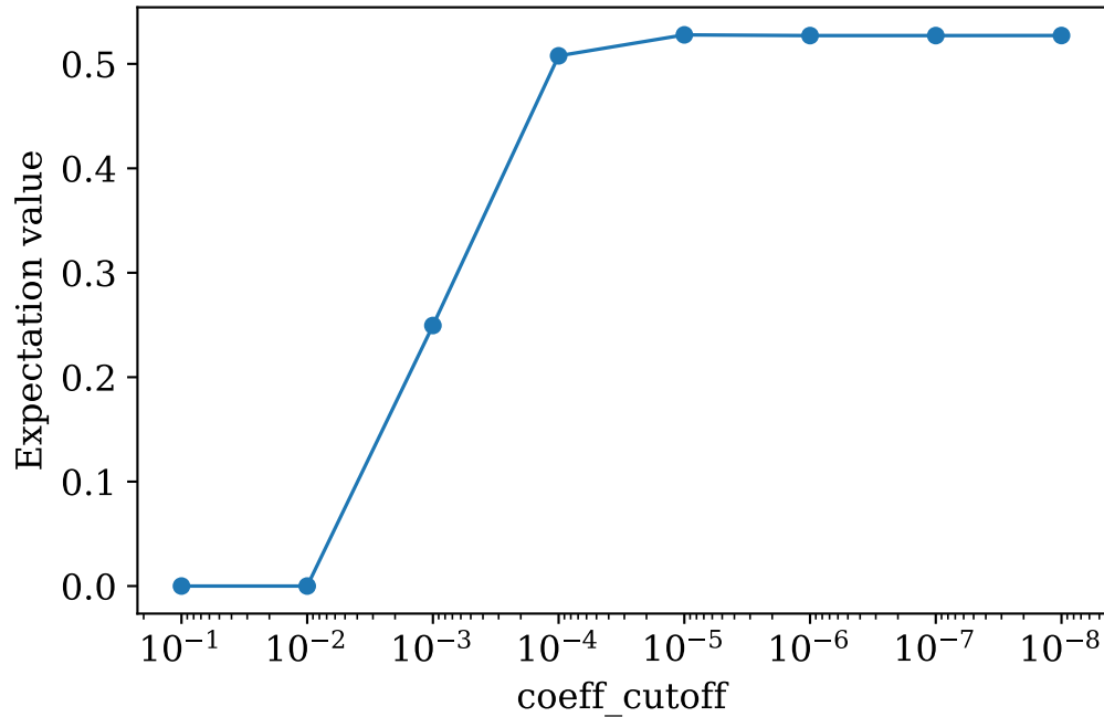
Z-string (w=2), damping=0.001
