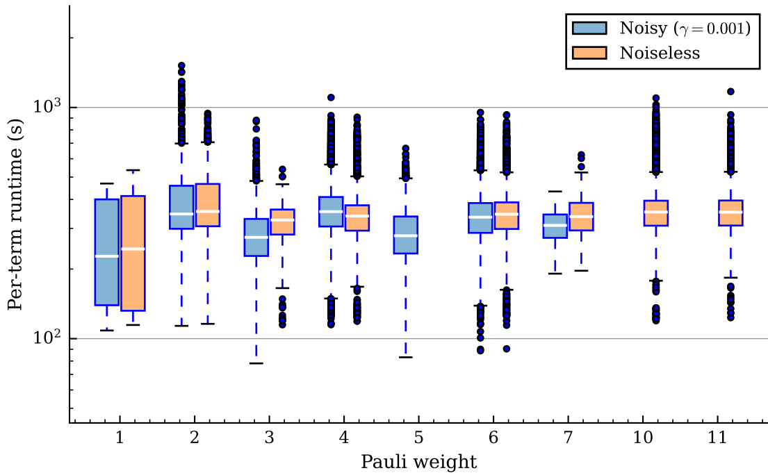
Per-term wall-clock runtime of FeS LUCJ ansatz propagation by Pauli weight
